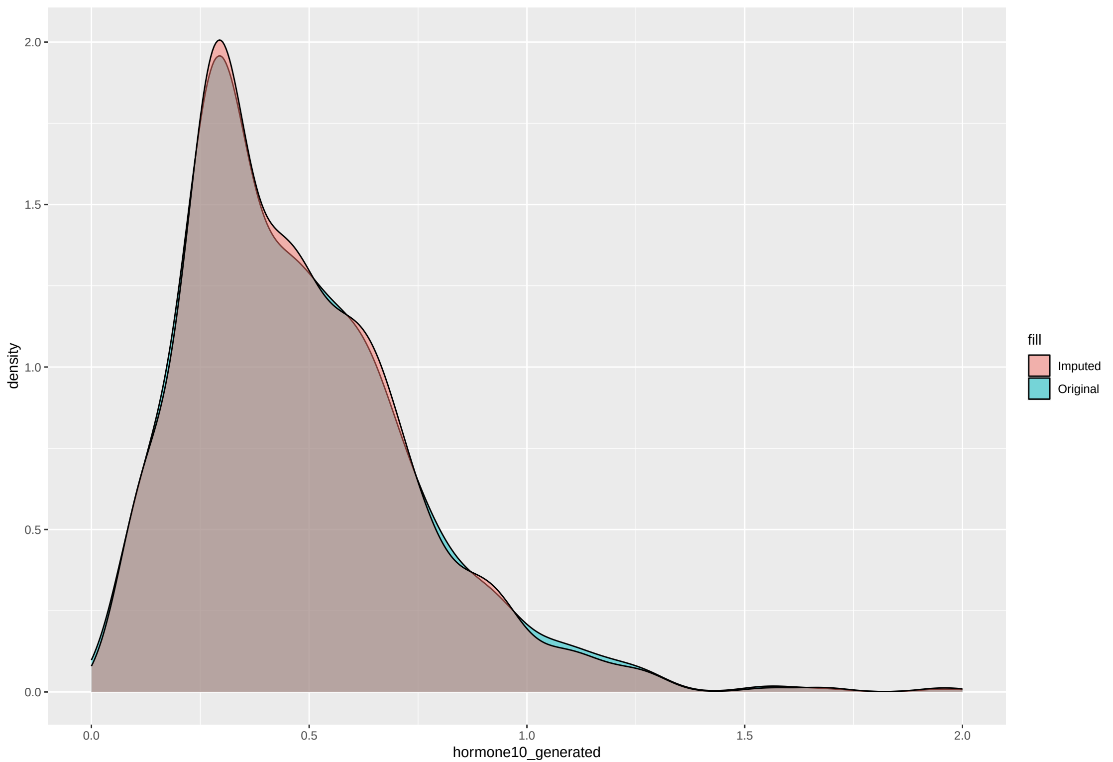
Density Plot of hormone10_generated: Original vs. Imputed
